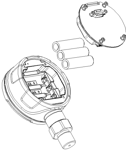
Figure 3 Install batteries
